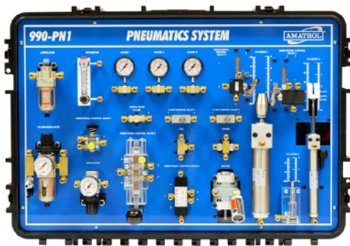
990-PN1 – Pneumatics
